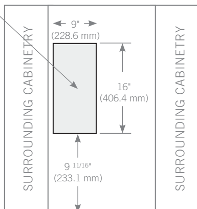
FRONT VIEW OF CABINERY OPENING
