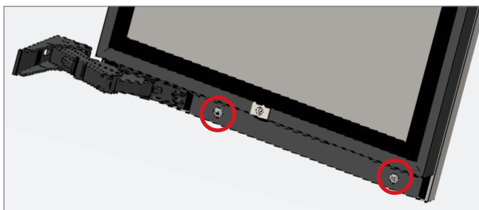
FIG. 2. Bottom door bracket screw locations.
